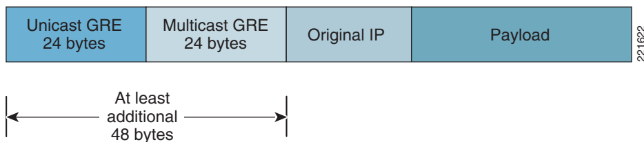
Figure 6-6 2547oDMVPN—Multicast Packet Overhead
