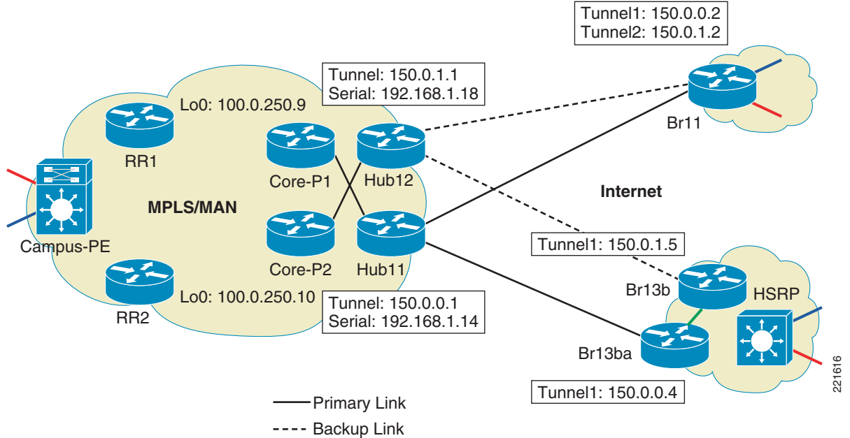
Figure 6-2 2547oDMVPN Redundancy
