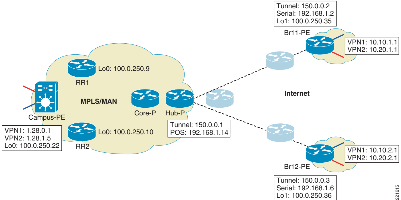
Figure 6-1 2547oDMVPN Deployment
