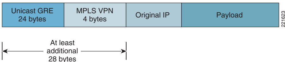
Figure 6-7 2547oDMVPN—Unicast Packet Overhead
